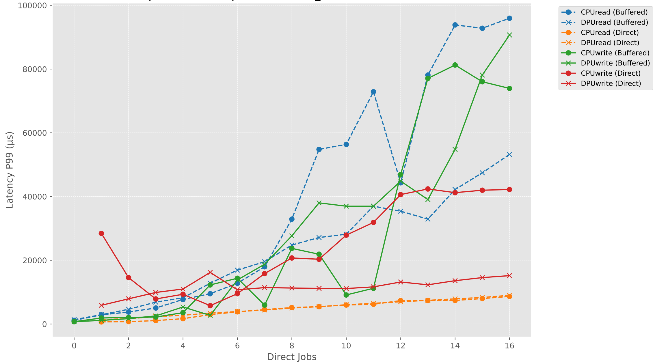
Latency P99 vs Direct Jobs (buffered1_directN) - SEQ (CPU vs DPU)
